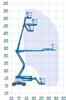
RANGE OF MOTION Z 45 -45/25J
