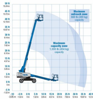
RANGE OF MOTION S 2 -40 XC™
